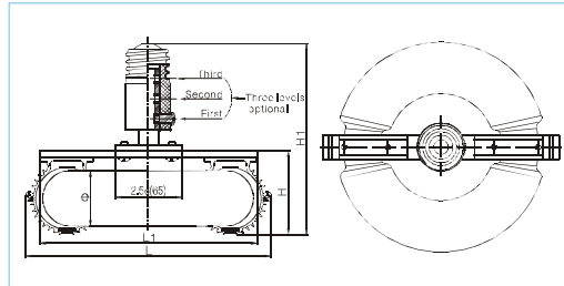
Dimensions [Unit: Inch(mm)]
